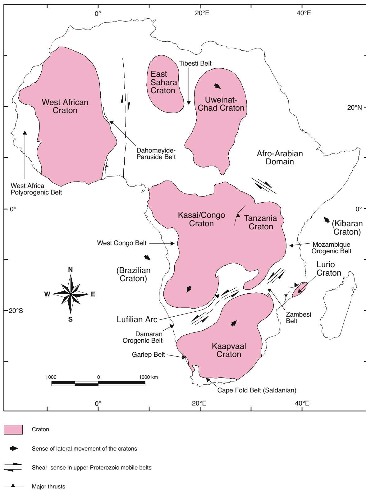
Fig. 6 Assumed extension of the Archean cratonic nuclei (after Key, 1992)
