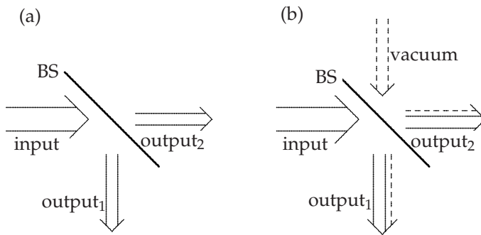
Fig. 1.3 Outline of the action of a 50%:50% beam splitter (BS). In classical optics (a) an incident light beam (input) is divided into two (apart from a phase shift) equal output beams ( \text{output}_1 , \text{output}_2 ). In quantum optics (b) the incident light beam and the quantum noise of the vacuum in the unused input port are combined to yield vacuum-noise-assisted output beams.
